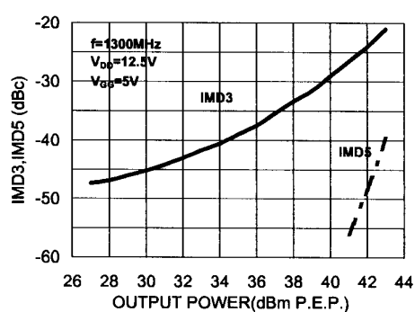
3rd,5th.INTERMODULATION DISTORTIN versus OUTPUT POWER CHARACTERISTICS
